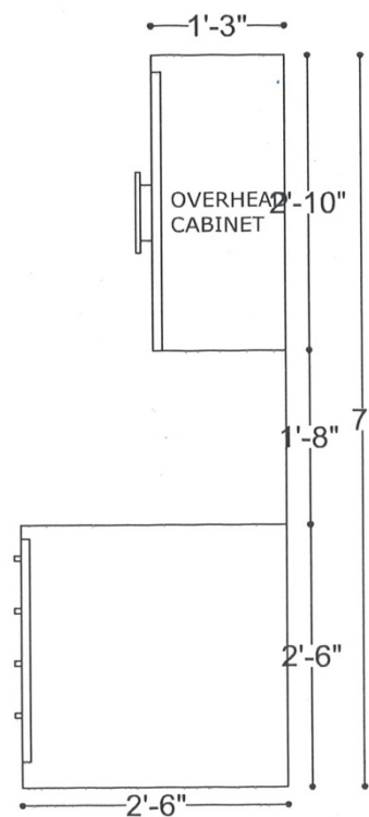
SIDE ELEVATION
